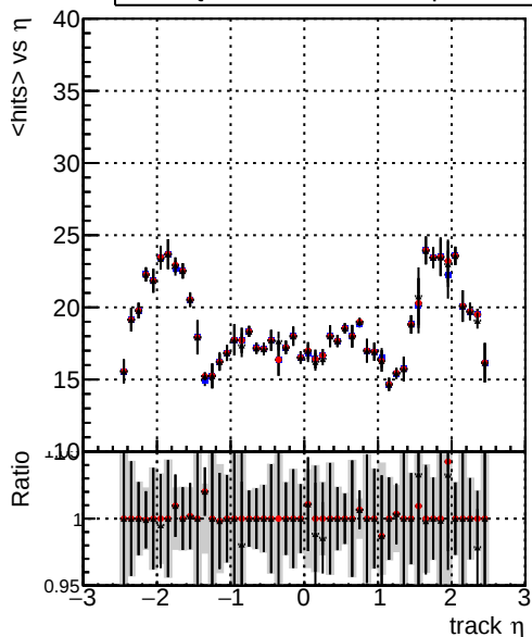
mean hits vs \eta — DQM_mkFit5_TTold-lowpt — DQM_mkFit_TT_retrain-lowpt — DQM_mkFit_TT_NEWdefault_specPLess3-lowpt
