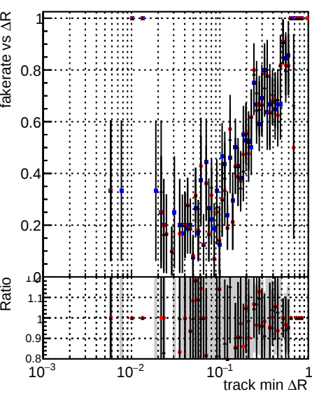
Fake rate vs \Delta R (track, jet) DQM_mkFit5_TTold-lowpt DQM_mkFit_TT_retrain-lowpt DQM_mkFit_TT_NEWdefault_specPLe3-lowpt
