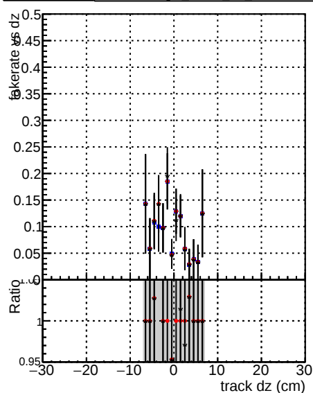
Fake rate vs dz Legend: DOM mkFit5 TTold-lowpnt DOM mkFit5 Tretain-lowpnt DOM mkFit5 TTNEWdefault specPless3-lowpnt
