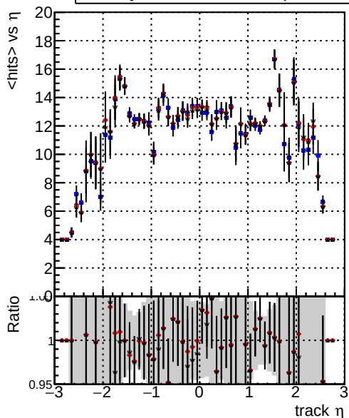
mean hit — DQM_mkFit5_TTold-lowpt — DQM_mkFit_TT_retrain-lowpt — DQM_mkFit_TT_NEWdefault_specPless3-lowpt
