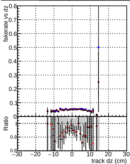
— DOM mkFit5 TTold-lowpt — DOM mkFit5 Ttrain-lowpt — DOM mkFit5 NEWdefault specPless3-lowpt
