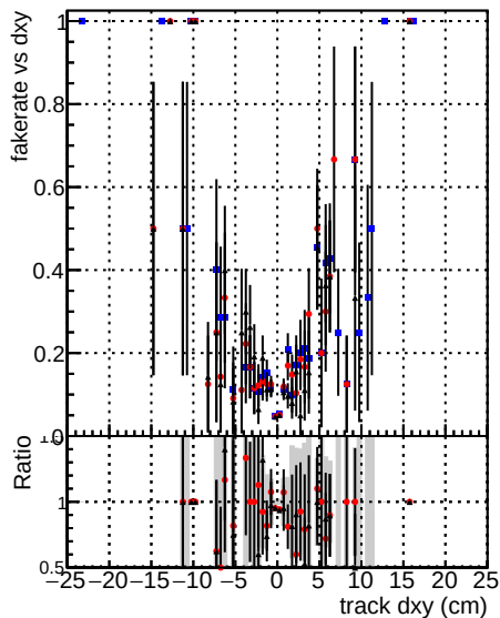
— DOM mkFit5 TTold-lowpt — DOM mkFit5 Ttrain-lowpt — DOM mkFit5 NEWdefault specPless3-lowpt
