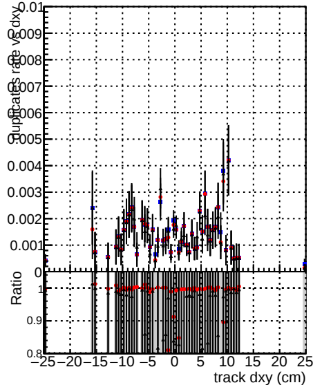
—●— DOM mkFit5 TTold-lowpt —●— DOM mkFit5 Tretain-lowpt —●— DOM mkFit5 TNEWdefault specPless3-lowpt
