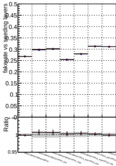
Fake rate vs. Legend: DOM mkFit5 TTold-lowpt DOM mkFit5 retain-lowpt DOM mkFit5 NEWdefault specPless3-lowpt
