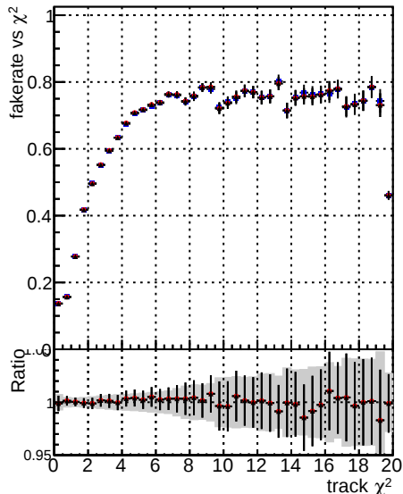
Fake rate vs. Legend: DOM mkFit5 TTold-lowpt DOM mkFit5 retain-lowpt DOM mkFit5 NEWdefault specPless3-lowpt
