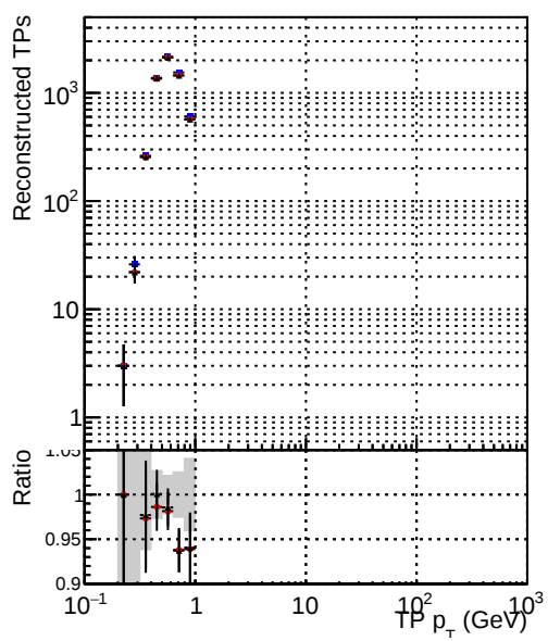
● DQM_mkFit5_TTold-lowpt ● DQM_mkFit_TT_retrain-lowpt ● DQM_mkFit_TT_NEWdefault_specPLess3-lowpt
