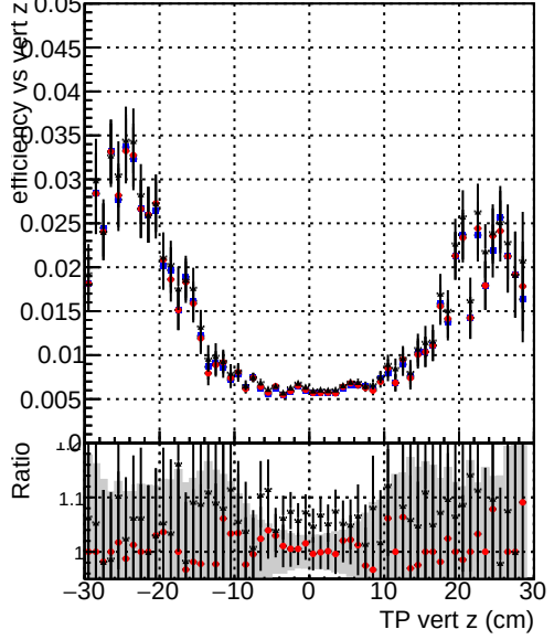
Efficiency vs. TP vert z — DQM_mkFit5_TTold-lowpt — DQM_mkFit_TT_retrain-lowpt — DQM_mkFit_TT_NEWdefault_specPLeSS3-lowpt
