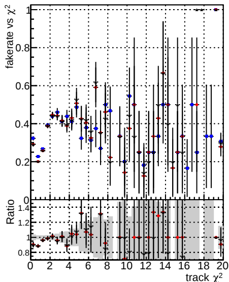
Fake rate vs. Legend: DOM mkFit5 Told-lowpt DOM mkFit Newdefault specPless3-lowpt
