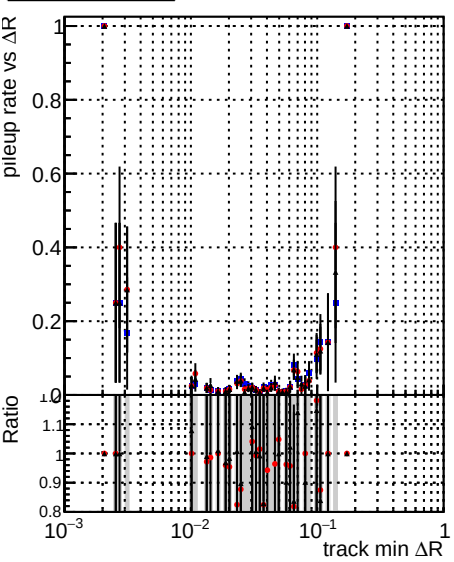
Legend: DQM_mkFit5_TTold-lowpt (blue circles), DQM_mkFit_TT_retrain-lowpt (red circles), DQM_mkFit_TT_NEWdefault_specPLe3-lowpt (black circles)
