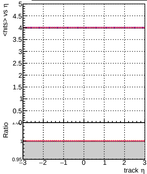
Legend: DOM mkFit XiminusNOPU NEWdefault specPless1, DOM mkFit XiminusNOPU NEWdefault specPless3, DOM mkFit XiminusNOPU NEWdefault specPless3, DOM mkFit XiminusNOPU NEWdefault specPless4
