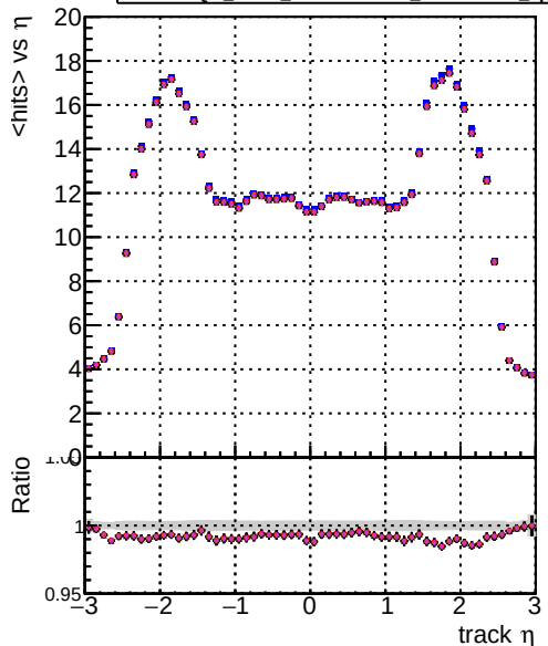
mean hit DOM mkFit XiminusNOPU NEWdefault specPless1 DOM mkFit XiminusNOPU NEWdefault specPless3 DOM mkFit XiminusNOPU NEWdefault specPless4
