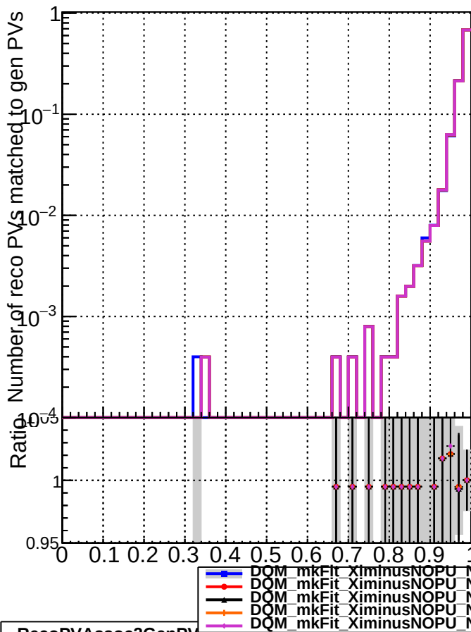
RecoPVAssoc2GenPVMatched_missing
