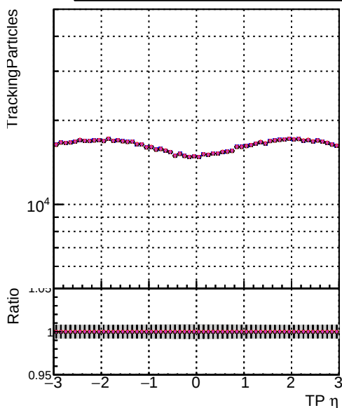
N of sim DOM mkFit XiminiusNOPU NEWdefault specPless2 DOM mkFit XiminiusNOPU NEWdefault specPless3
