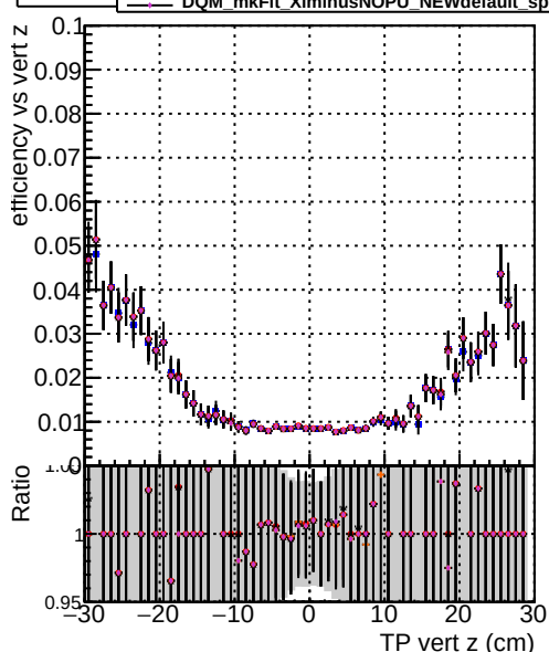
Efficiency Model Method Configuration Spec PLess2 PLess3 PLess4 DOM mkFit Ximinus NOPU NEWdefault spec PLess2 DOM mkFit Ximinus NOPU NEWdefault spec PLess3 DOM mkFit Ximinus NOPU NEWdefault spec PLess4
