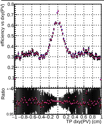
Efficiency vs Dxy(PV) (TP dxy(PV) (cm)) fake+duplicates vs dxy(PV) (track dxy(PV) (cm))
