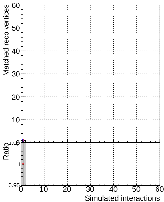
MatchedRecoVtx_vs_GenVtx
