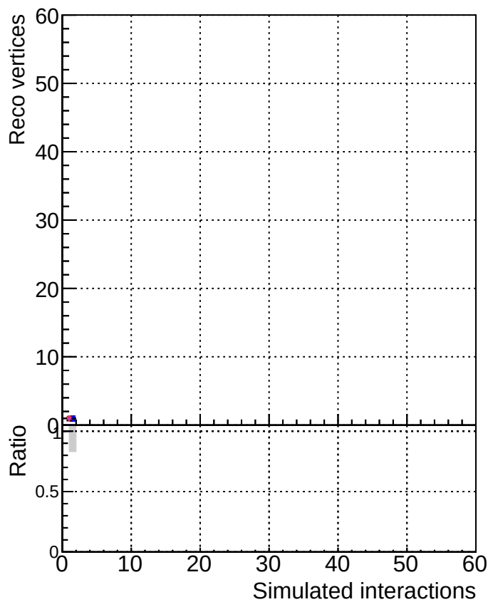
RecoVtx_vs_GenVtx
