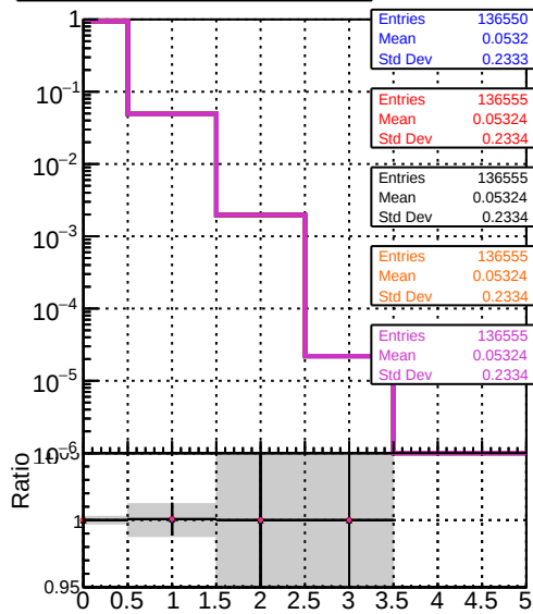
Legend: DOM mkFit XiminusNOPU NEWdefault specPless1 specPless2 specPless3 specPless4 mean hit
