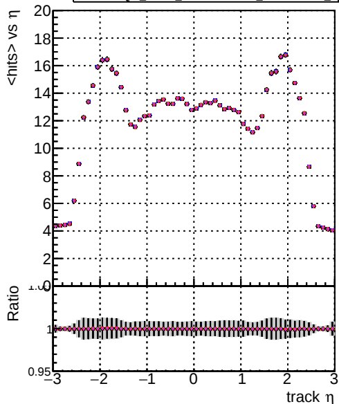
Legend: DOM mkFit XiminusNOPU NEWdefault specPless1 specPless2 specPless3 specPless4 mean hit
