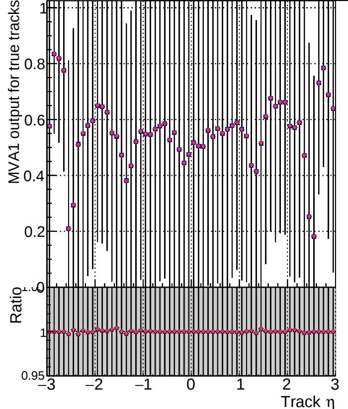
MVA1 of associated tracks (recoToSim) vs. track \eta Legend: DOM mkFit XiminusNOPU NEWdefault specPless1 DOM mkFit XiminusNOPU NEWdefault specPless2 DOM mkFit XiminusNOPU NEWdefault specPless3 DOM mkFit XiminusNOPU NEWdefault specPless4
