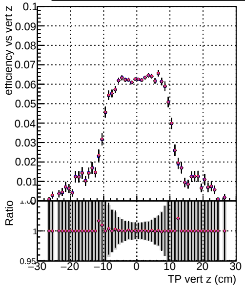
Efficiency vs. TP vert z (cm) DOM mkFit XiminusNOPU NEWdefault specPless3 DOM mkFit XiminusNOPU NEWdefault specPless4 DOM mkFit XiminusNOPU NEWdefault specPless3 DOM mkFit XiminusNOPU NEWdefault specPless4
