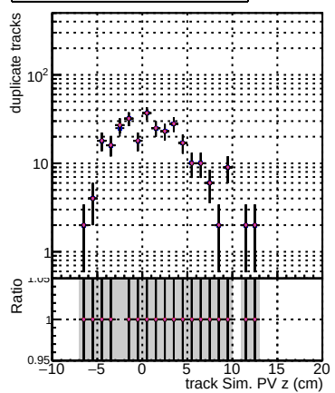
N of associated tracks (recoToSim) looper tracks vs. sim PV z
