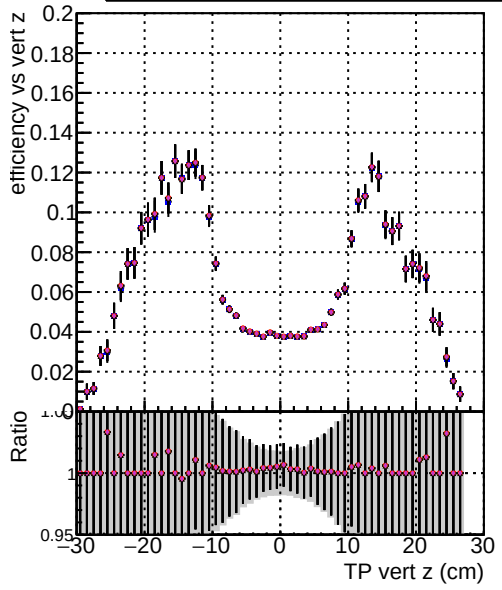
Efficiency vs. sim PV z DOM mkFit XiminusNOPU NEWdefault specPless1 DOM mkFit XiminusNOPU NEWdefault specPless3 DOM mkFit XiminusNOPU NEWdefault specPless4
