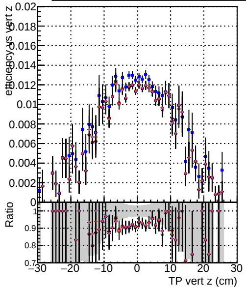
Efficiency vs. TP vert z (cm) DOM mkFit Ximinus NOPU NEWdefault specPless1 DOM mkFit Ximinus NOPU NEWdefault specPless3 DOM mkFit Ximinus NOPU NEWdefault specPless4
