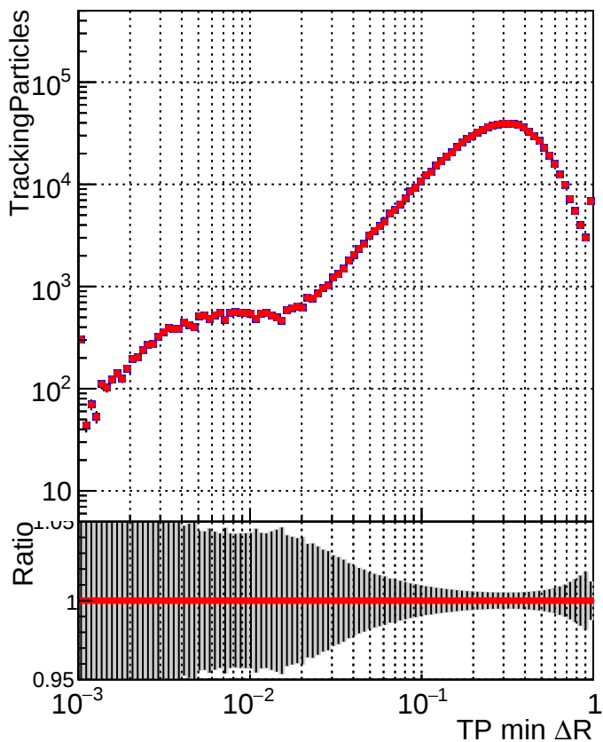
N of simulated tracks vs ΔR(TP, jet)
