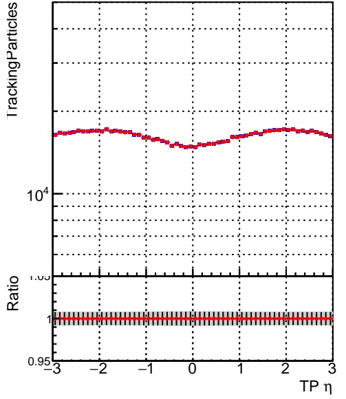
N of simulated tracks vs TP \eta ■ DQM_mkFit_XiminusNOPU_NEWdefault ■ DQM_mkFit_XiminusNOPU_OLD6iters
