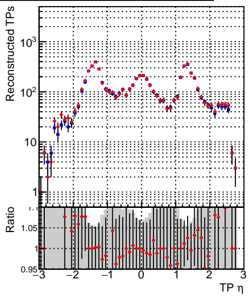
Legend: DQM_mkFit_XiminusNOPU_NEWdefault (blue squares), DQM_mkFit_XiminusNOPU_OLD6iters (red circles)
