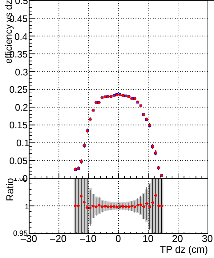
Efficiency vs Dz Legend: DQM_mkFit_XiminusNOPU_NEWdefault DQM_mkFit_XiminusNOPU_OLD6iters
