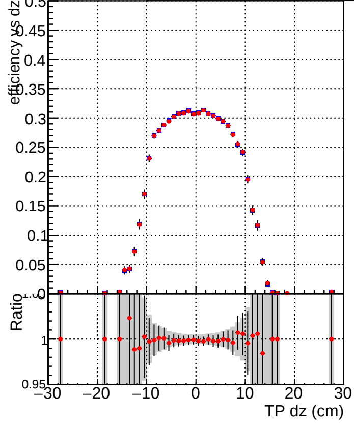
Efficiency vs Dz Legend: DQM_mkFit_XiminusNOPU_NEWdefault (Blue squares) DQM_mkFit_XiminusNOPU_OLD6iters (Red circles)
