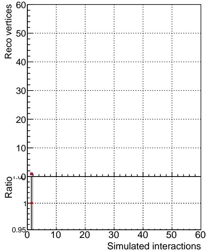
RecoVtx_vs_GenVtx
