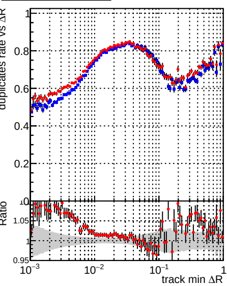
Legend: DQM_mkFit_XiminusNOPU_NEWdefault (blue line with error bars), DQM_mkFit_XiminusNOPU_OLD6iters (red line with error bars)
