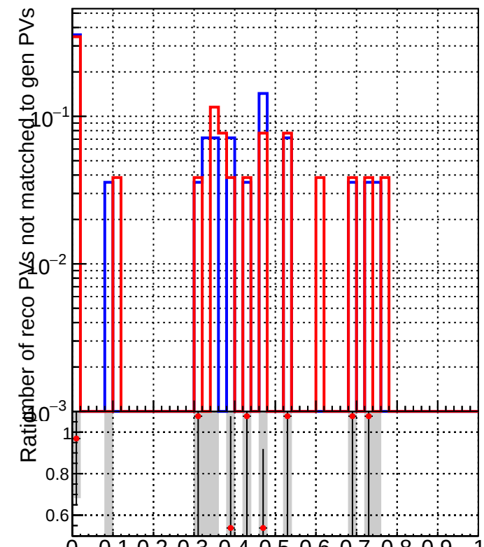
RecoPVAssoc2GenPVnotmatched_missing
