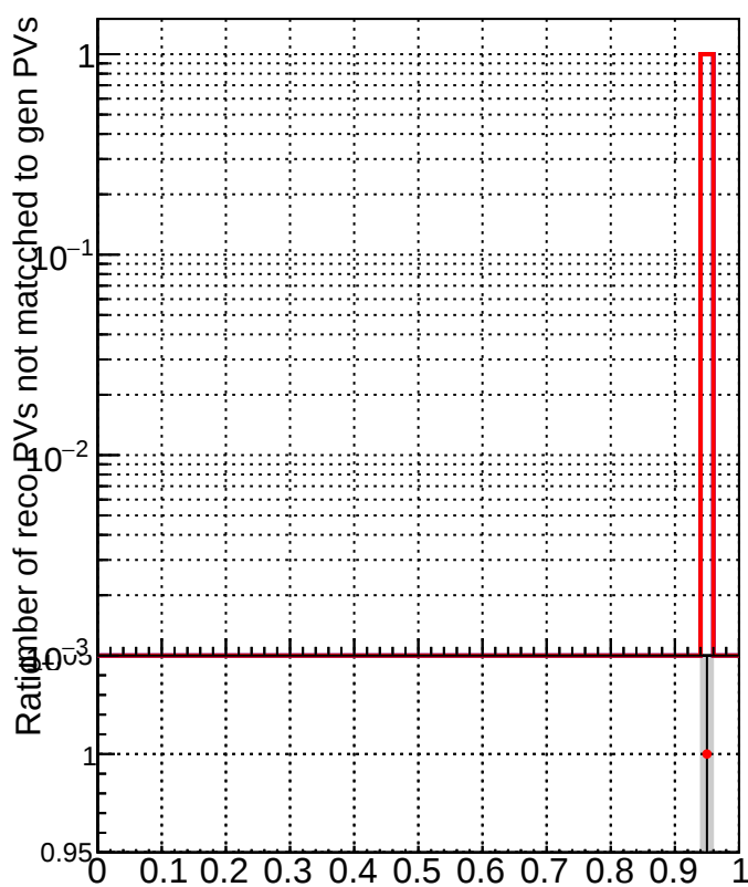
RecoPVAssoc2GenPVNotMatched_Purity
