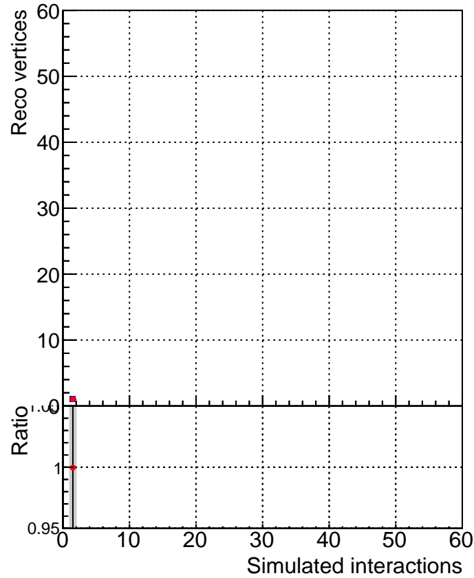
RecoVtx_vs_GenVtx
