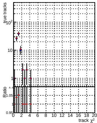
N of reco track vs. \chi^2 for DQM mkFit XiminusNOPU_NEWdefault and DQM mkFit XiminusNOPU_OLD6iters
