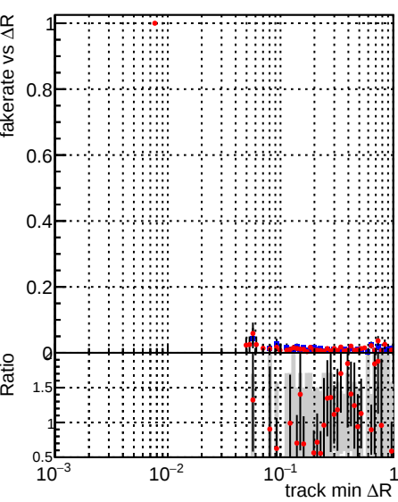
Legend: DQM_mkFit_XiminusNOPU_NEWdefault (grey line with blue dots), DQM_mkFit_XiminusNOPU_OLD6iters (red line with red dots)
