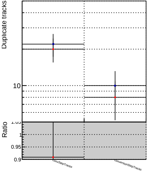
Number of tracks vs collection Legend: DQM_mkFit_XiminusNOPU_NEWdefault (Blue square) DQM_mkFit_XiminusNOPU_OLD6iters (Red circle)
