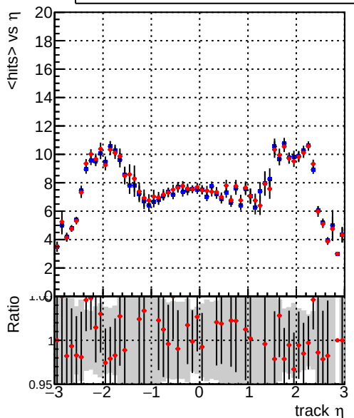
mean hits vs \eta Legend: DQM_mkFit_XiminusNOPU_NEWdefault (blue line), DQM_mkFit_XiminusNOPU_OLD6iters (red line)
