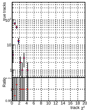
N of reco track vs. \chi^2 for DQM mkFit XiminusNOPU_NEWdefault (black) and DQM mkFit XiminusNOPU_OLD6iters (red).
