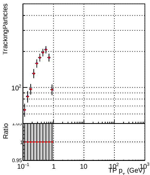
N of sim —●— DOM_mkFit_XiminusNOPU_OLD6iters
