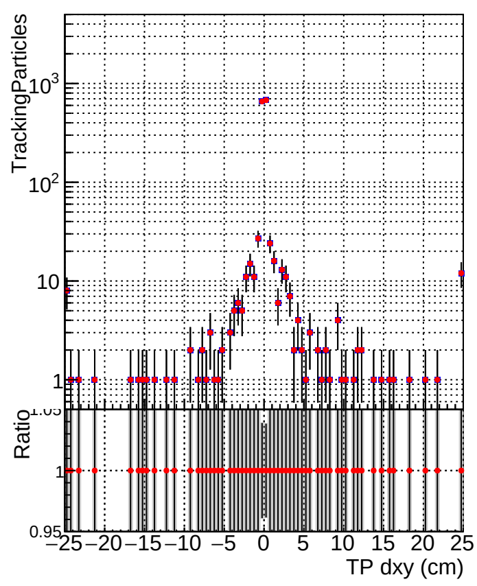
N of simulated track Legend: DQM_mkFit_XiminusNOPU_NEWdefault DQM_mkFit_XiminusNOPU_OLD6iters
