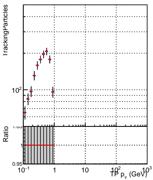
Legend for Ratio vs pT plots: Blue square: DQM_mkFit_XiminusNOPU_NEWdefault Red circle: DQM_mkFit_XiminusNOPU_OLD6iters
