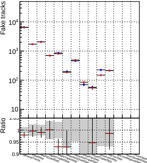
Number —●— DQM_mkFit_XiminusNOPU_OLD6iters
