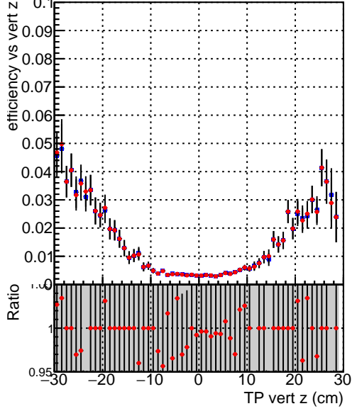
Efficiency vs. TP vert z (cm) Legend: — DQM_mkFit_XiminusNOPU_NEWdefault (blue squares) — DQM_mkFit_XiminusNOPU_OLD6iters (red crosses)
