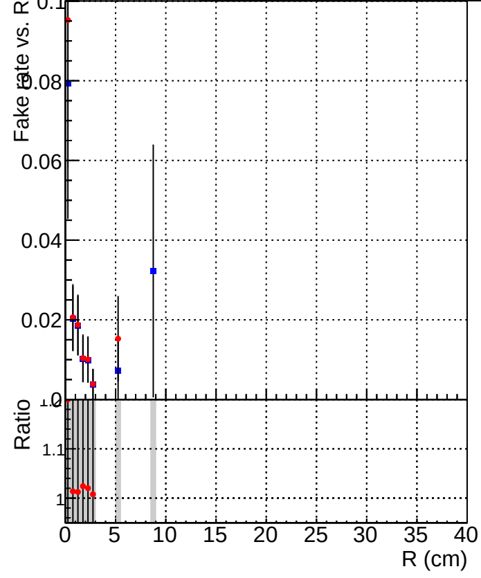
K_S^0 tracking fake rate vs R Legend: DQM_mkFit_XiminusNOPU_NEWdefault (blue squares) DQM_mkFit_XiminusNOPU_OLD6iters (red circles)
