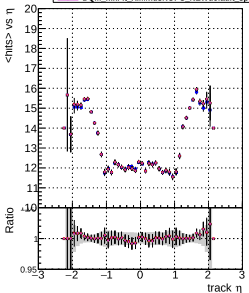
Legend: DOM mkFit XiMinusNOPU NEWdefault specPless5, DOM mkFit XiMinusNOPU NEWdefault specPless3, DOM mkFit XiMinusNOPU NEWdefault specPless3, DOM mkFit XiMinusNOPU NEWdefault specPless4 mean hits
