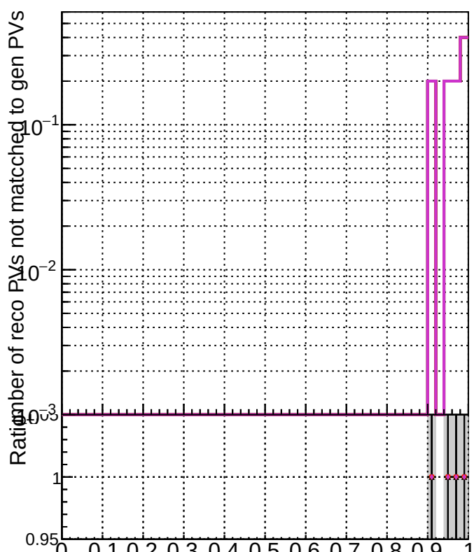
RecoPVAssoc2GenPVNotMatched_Purity
