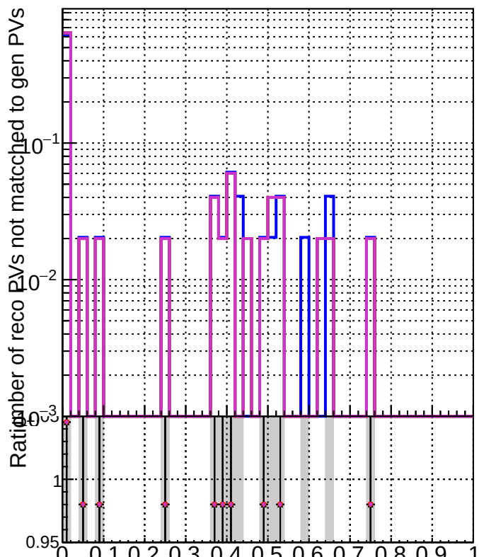
RecoPVAssoc2GenPVnotmatched_missing
