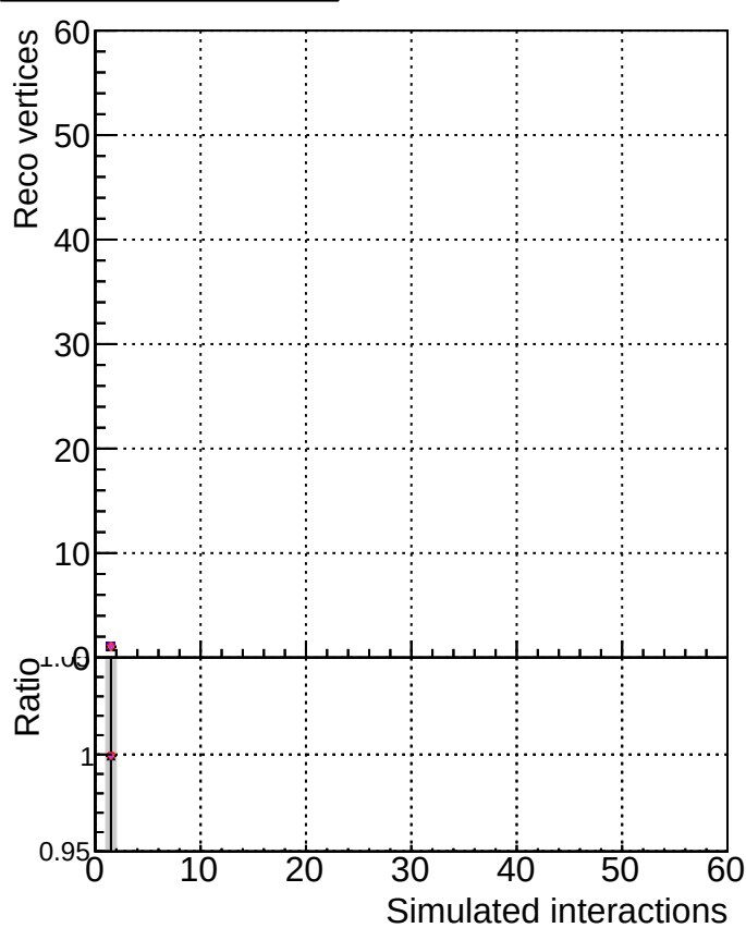
RecoVtx_vs_GenVtx
