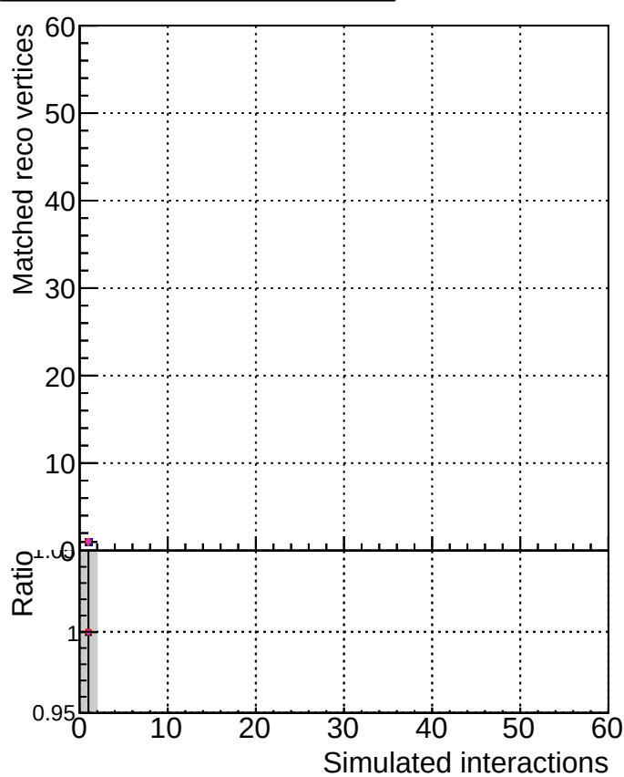
MatchedRecoVtx_vs_GenVtx
