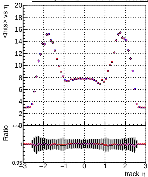
mean hit DOM mkFit XiMinusNOPU NEWdefault specPless1 DOM mkFit XiMinusNOPU NEWdefault specPless3 DOM mkFit XiMinusNOPU NEWdefault specPless3 DOM mkFit XiMinusNOPU NEWdefault specPless4
