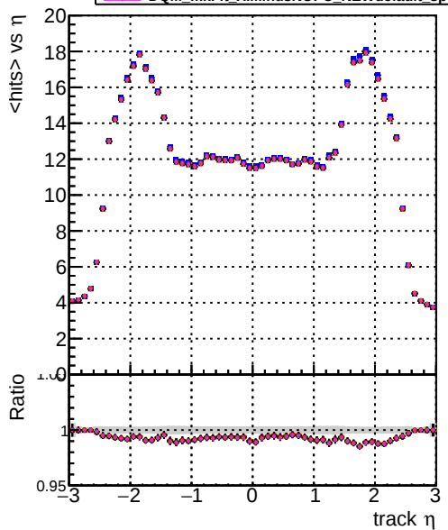
Legend: DOM mkFit XiMinusNOPU NEWdefault specPless1, DOM mkFit XiMinusNOPU NEWdefault specPless3, DOM mkFit XiMinusNOPU NEWdefault specPless4 mean hit
