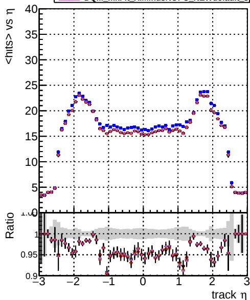
mean hit DOM mkFit XiMinusNOPU NEWdefault specPless1 DOM mkFit XiMinusNOPU NEWdefault specPless3 DOM mkFit XiMinusNOPU NEWdefault specPless4
